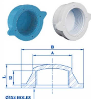
Ø3X4 HOLES
