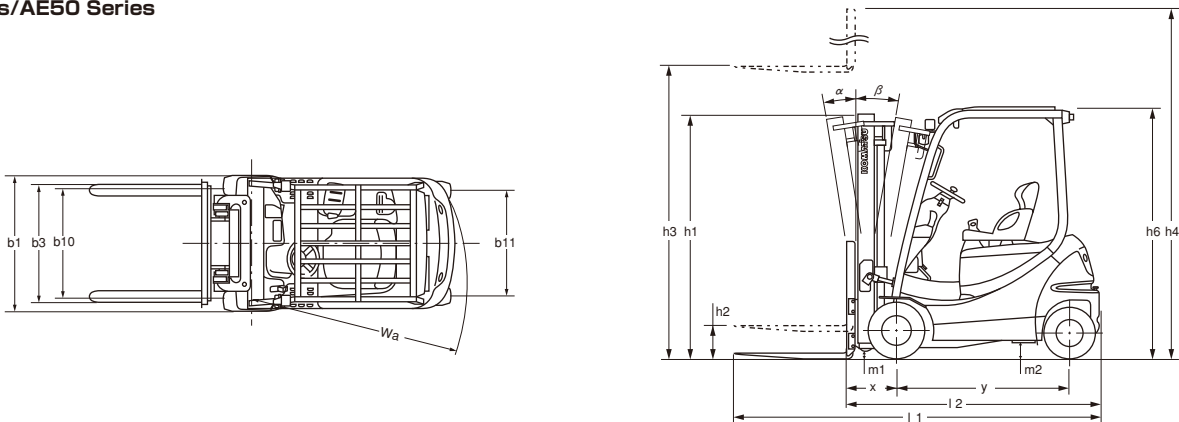
■Dimensions/AE50 Series
