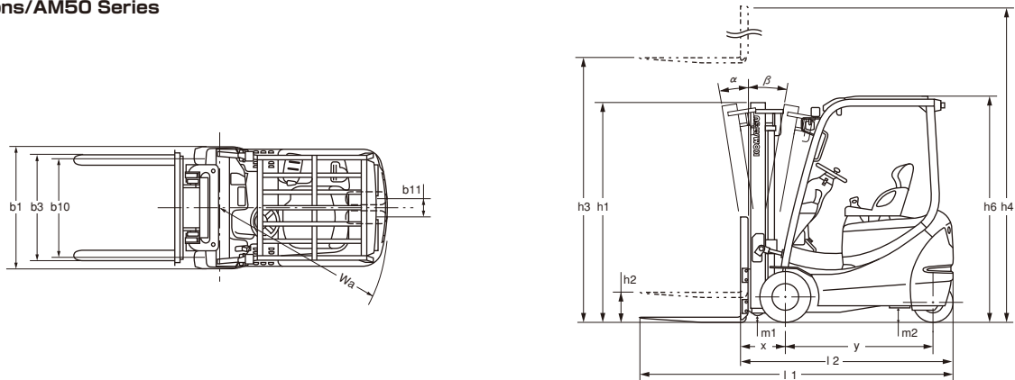
■Dimensions/AM50 Series
